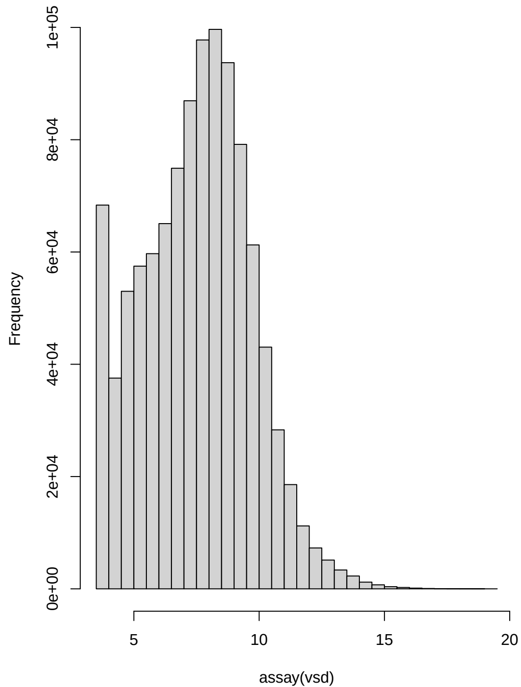
Histogram of assay(vsd)
